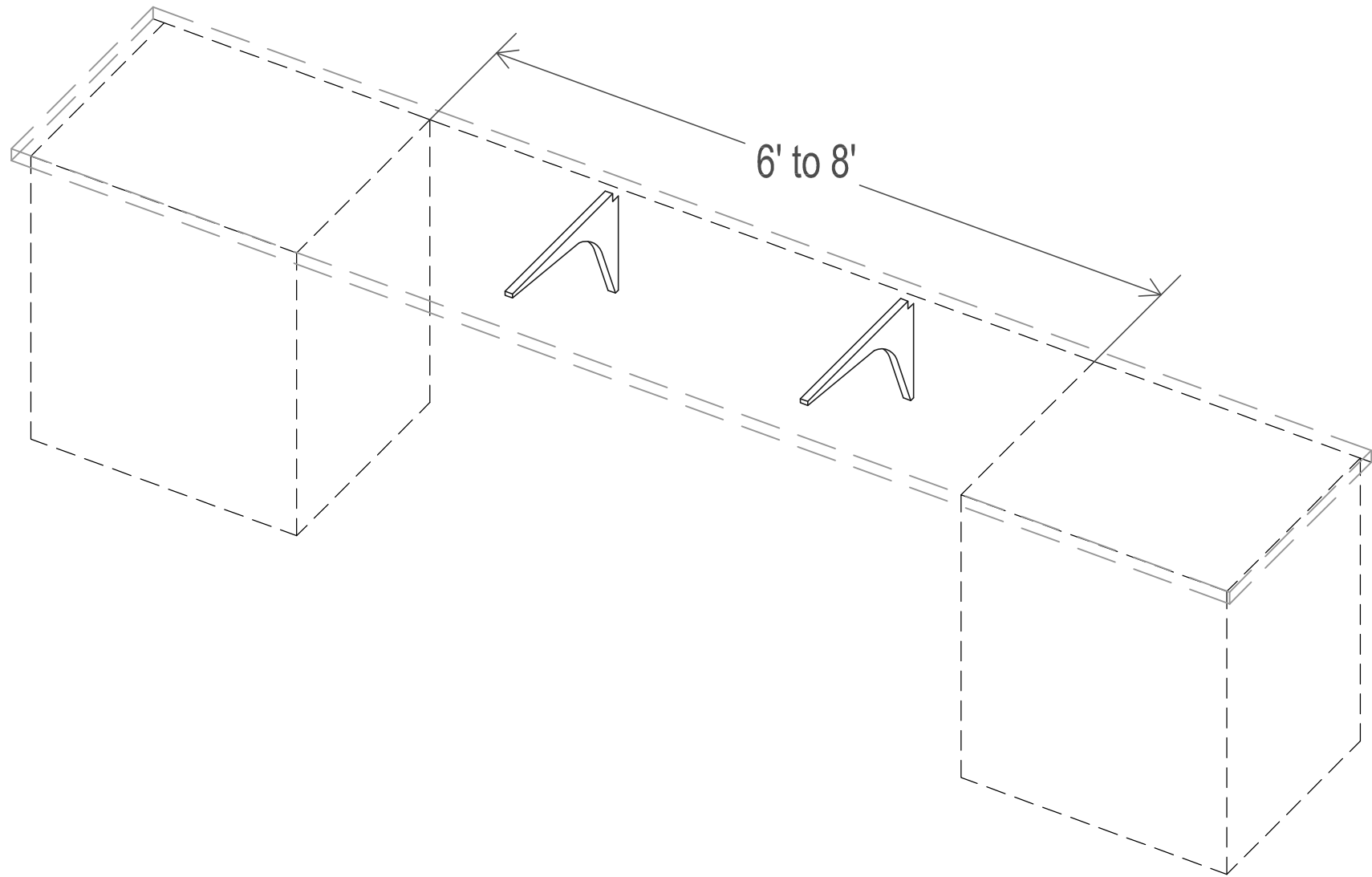
#07 Adjustable Easy Bracket Support
